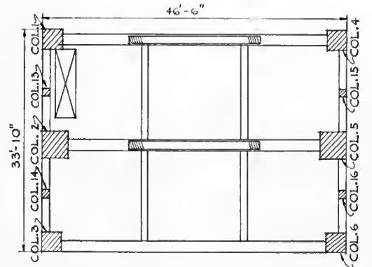
SECTION B-B. PLAN OF SECOND FLOOR
